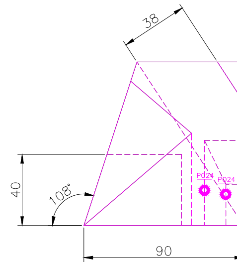
RIGHT SCALE 1/2
