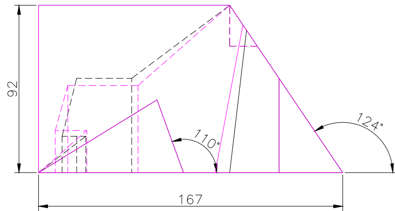
FRONT SCALE 1/2
