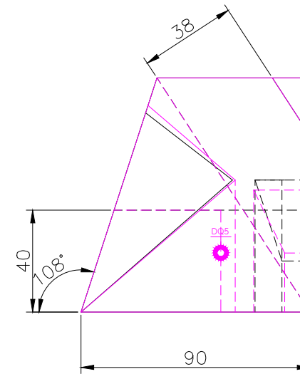
RIGHT SCALE 1/2
