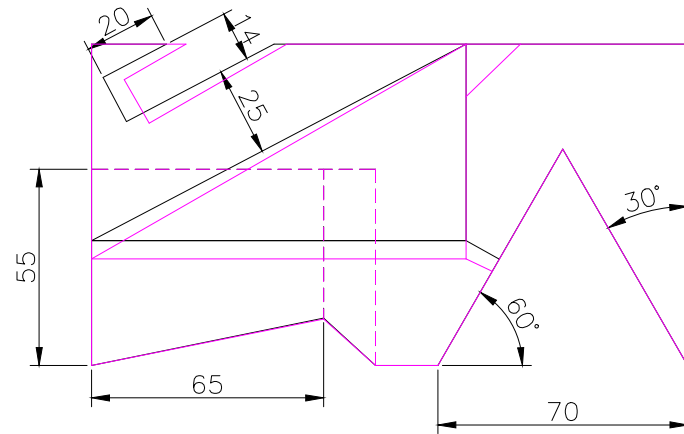
TOP SCALE 1/2
