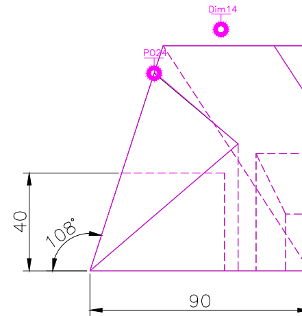
RIGHT SCALE 1/2
