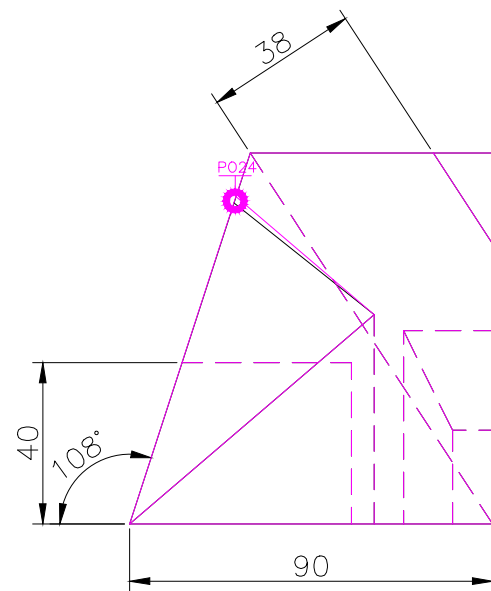
RIGHT SCALE 1/2
