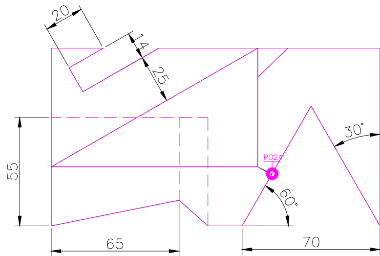
TOP SCALE 1/2
