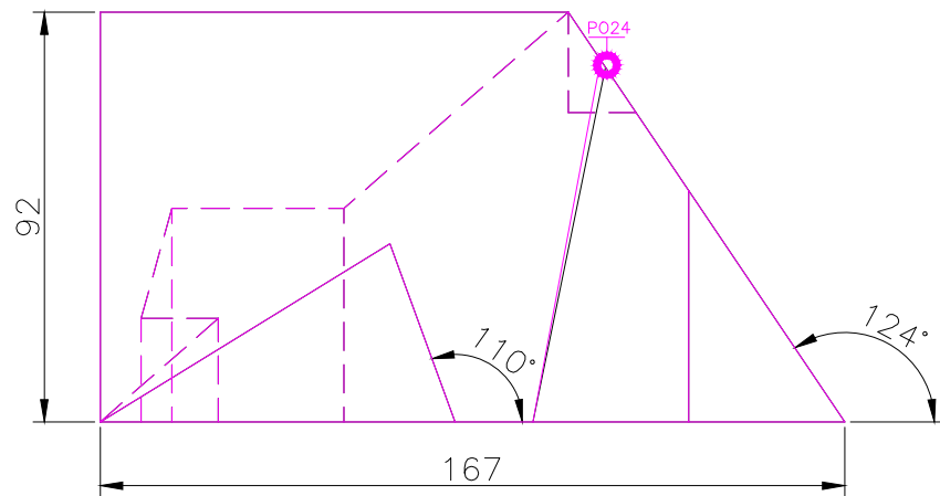
FRONT SCALE 1/2
