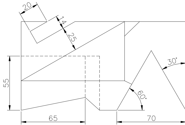
TOP SCALE 1/2
