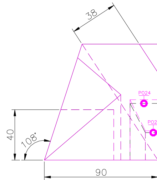
RIGHT SCALE 1/2
