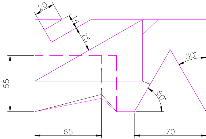
TOP SCALE 1/2
