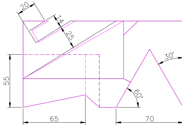
TOP SCALE 1/2
