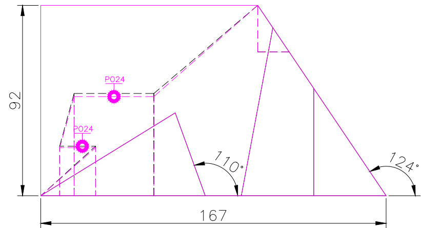
FRONT SCALE 1/2
