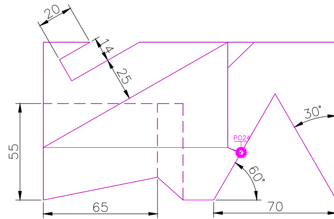
TOP SCALE 1/2
