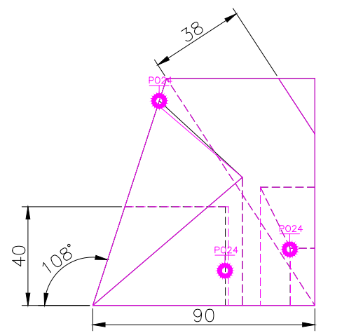
RIGHT SCALE 1/2
