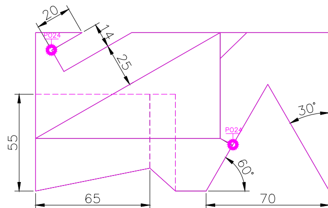
TOP SCALE 1/2
