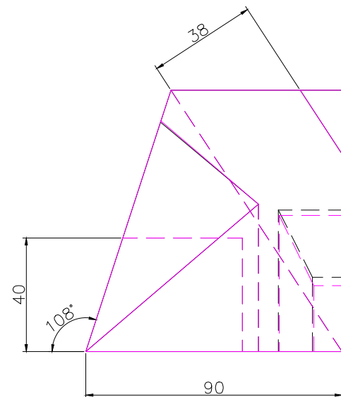
RIGHT SCALE 1/2
