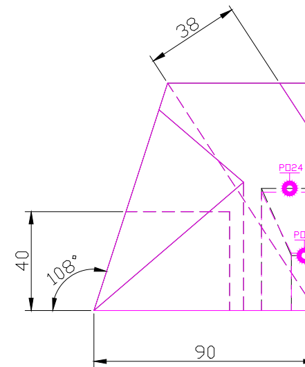
RIGHT SCALE 1/2
