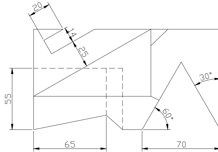
TOP SCALE 1/2
