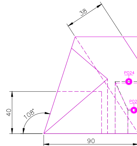
RIGHT SCALE 1/2
