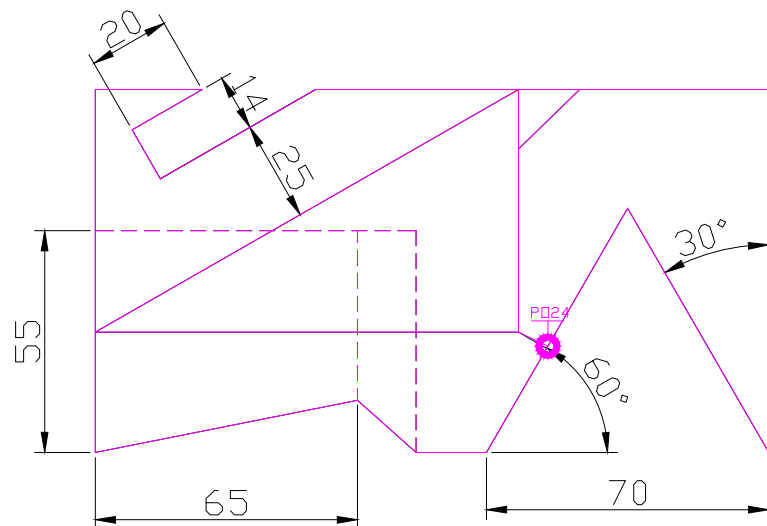
TOP SCALE 1/2
