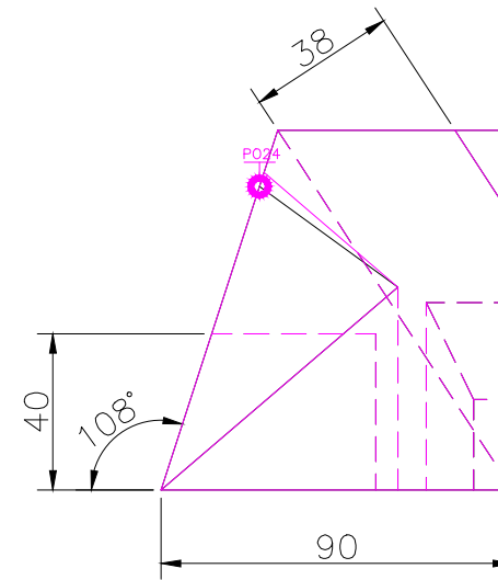
RIGHT SCALE 1/2
