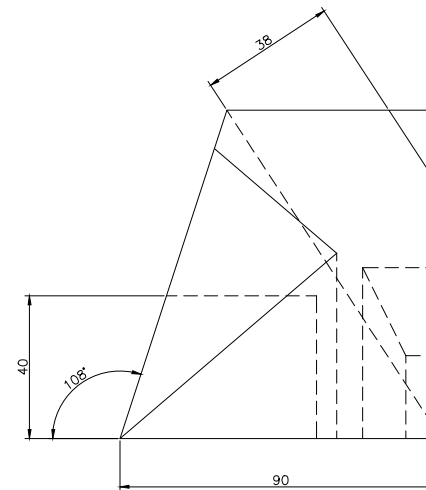
RIGHT SCALE 1/2
