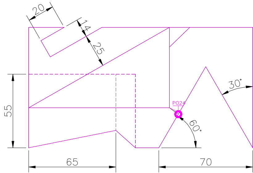
TOP SCALE 1/2
