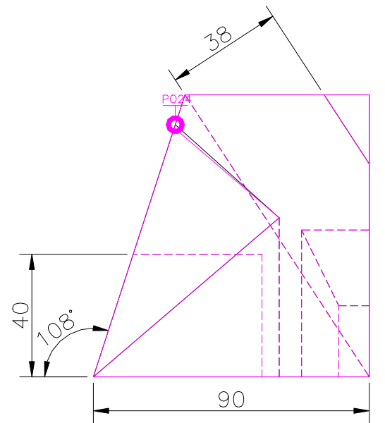
RIGHT SCALE 1/2
