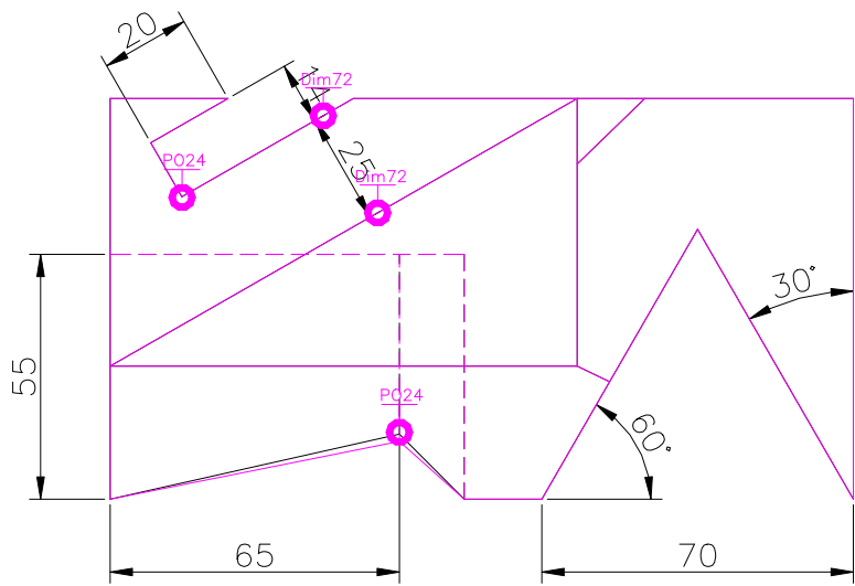
TOP SCALE 1/2
