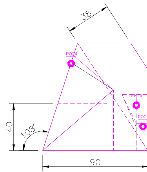
RIGHT SCALE 1/2
