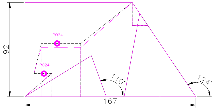
FRONT SCALE 1/2
