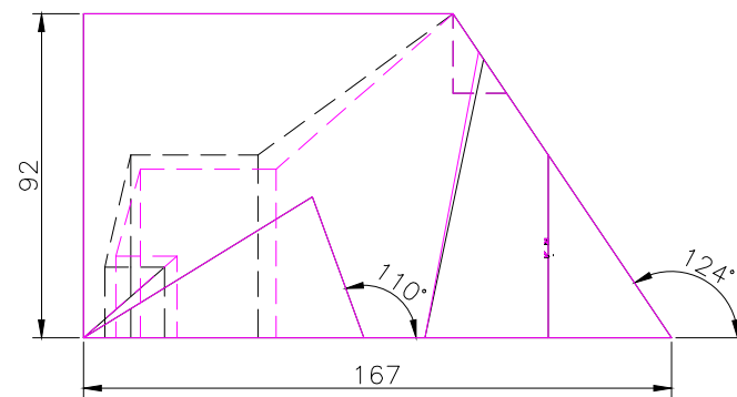
FRONT SCALE 1/2
