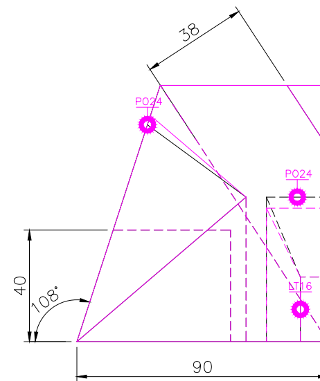
RIGHT SCALE 1/2
