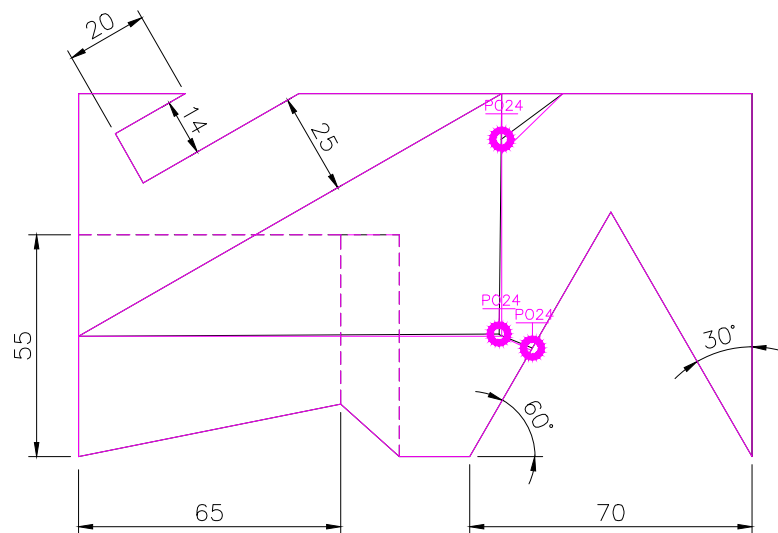
TOP SCALE 1/2
