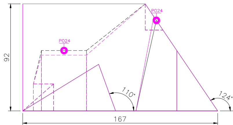
FRONT SCALE 1/2
