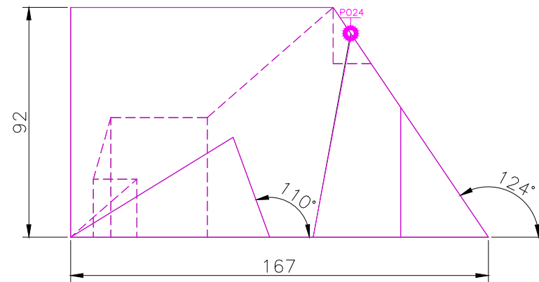
FRONT SCALE 1/2
