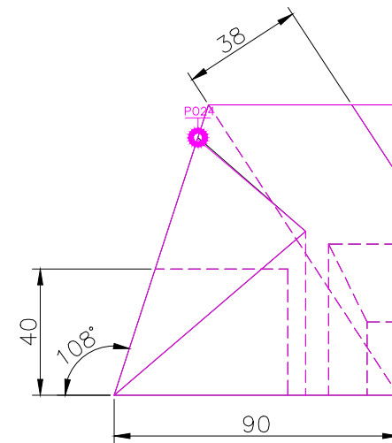
RIGHT SCALE 1/2
