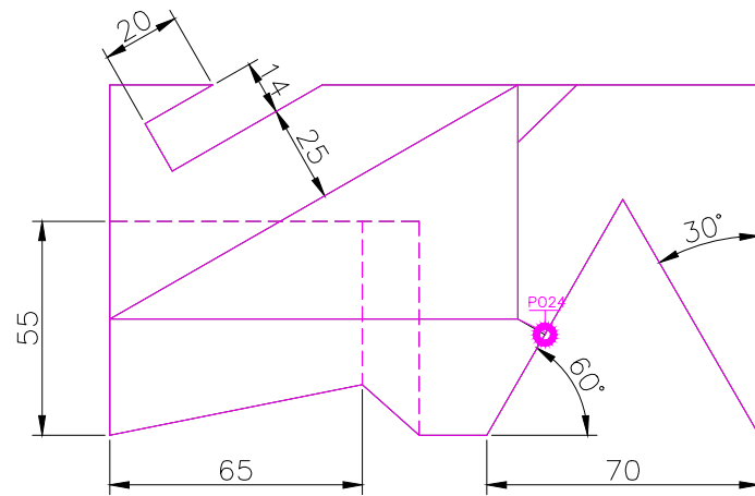
TOP SCALE 1/2
