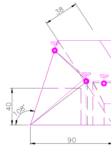
RIGHT scal 1/2
