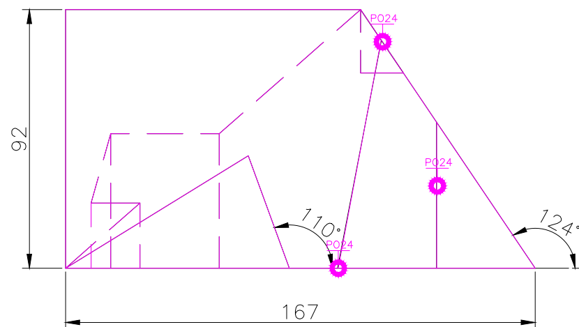
FRONT scal 1/2
