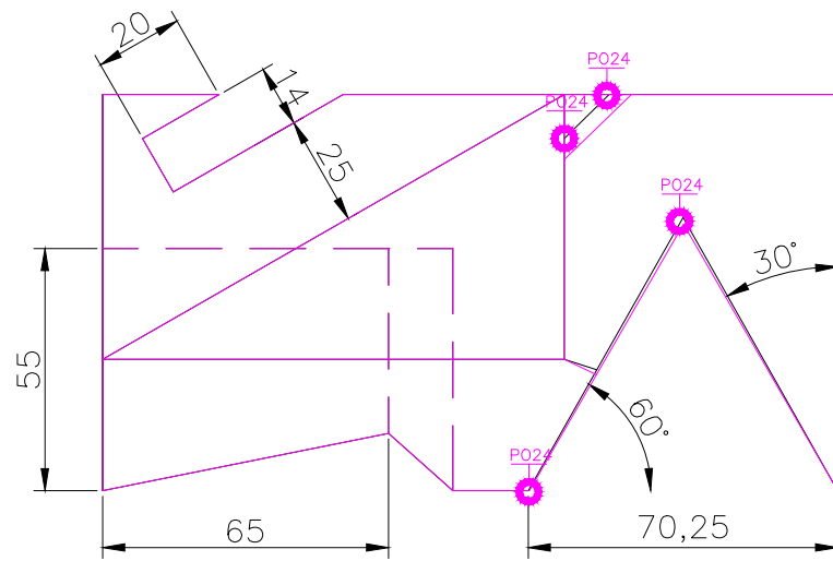
TOP scal 1/2
