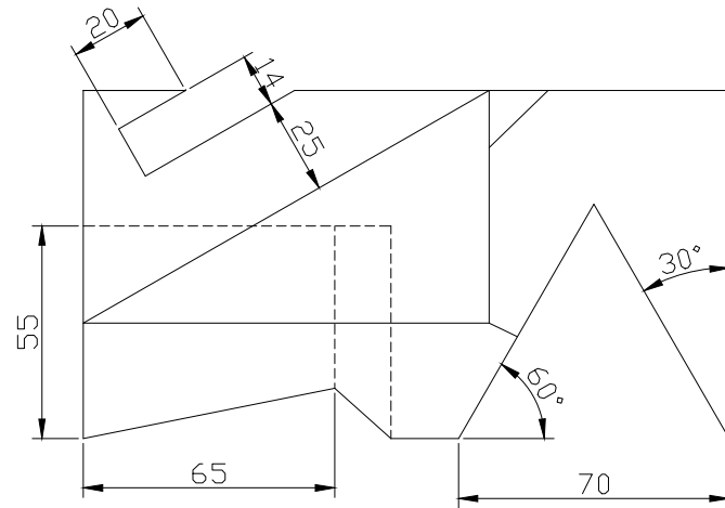
TOP SCALE 1/2
