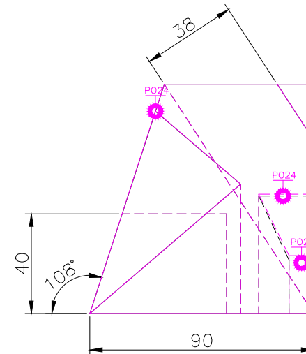
RIGHT SCALE 1/2
