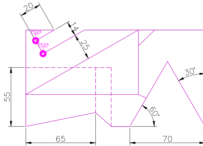
TOP SCALE 1/2
