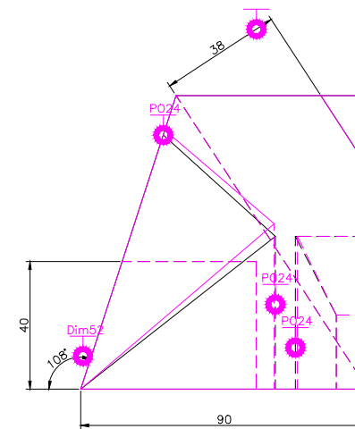
RIGHT SCALE 1/2
