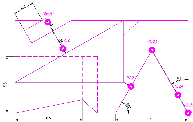
TOP SCALE 1/2
