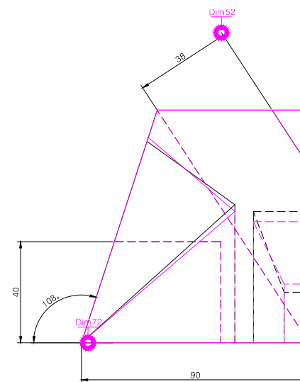
RIGHT SCALE 1/2
