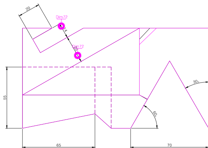
TOP SCALE 1/2
