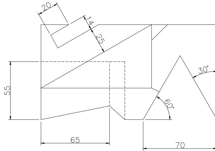
TOP SCALE 1/2
