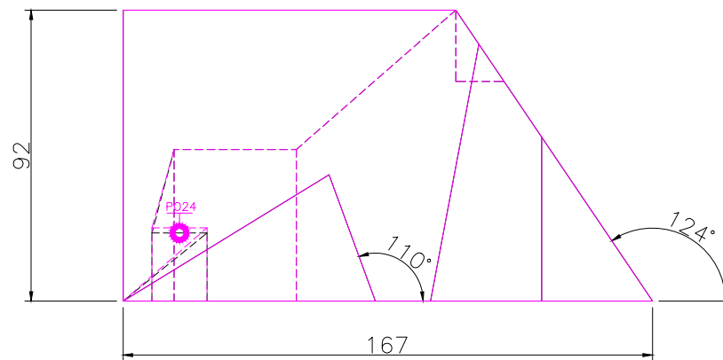
FRONT SCALE 1/2
