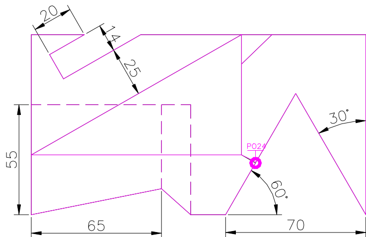
TOP SCALE 1/2
