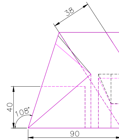
RIGHT SCALE 1/2
