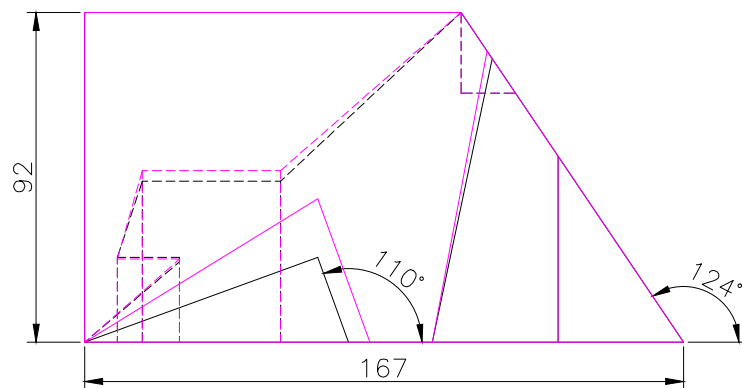
FRONT SCALE 1/2
