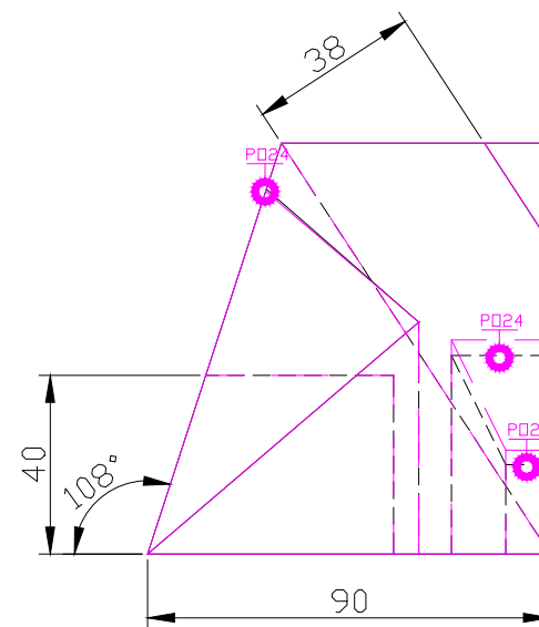
RIGHT SCALE 1/2
