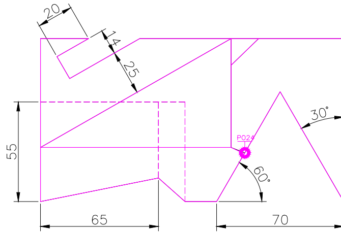
TOP SCALE 1/2
