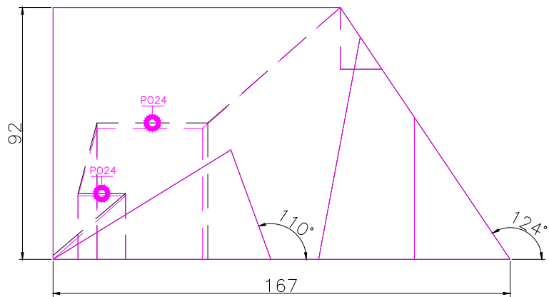
FRONT SCALE 1/2
