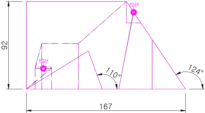
FRONT SCALE 1/2
