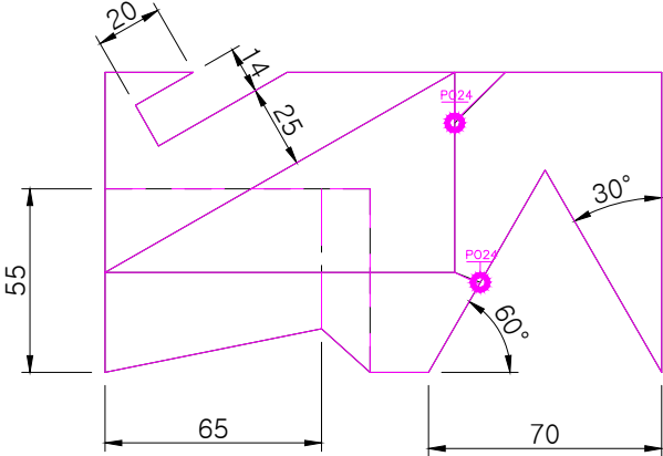
TOP SCALE 1/2
