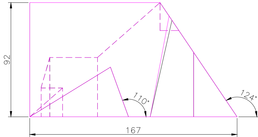
FRONT SCALE 1/2
