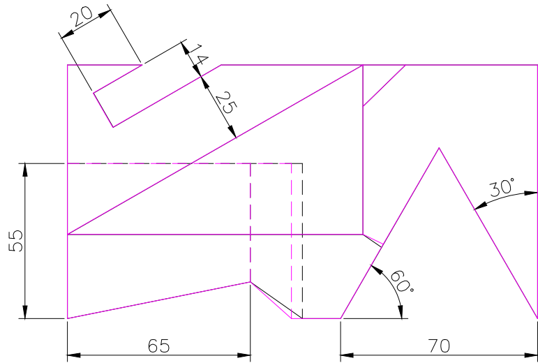
TOP SCALE 1/2
