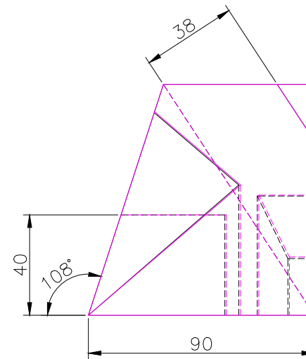
RIGHT SCALE 1/2
