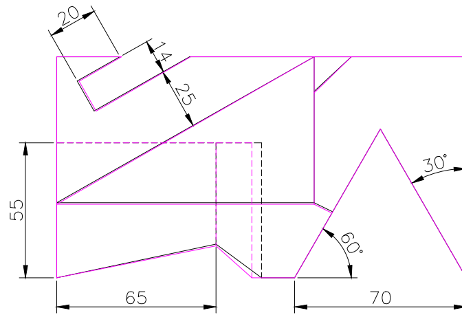
TOP SCALE 1/2
