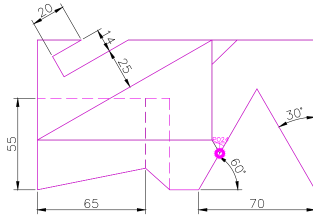
TOP SCALE 1/2
