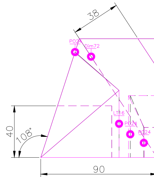
RIGHT SCALE 1/2
