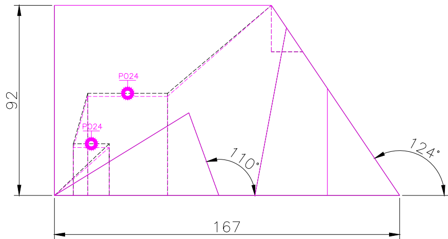
FRONT SCALE 1/2
