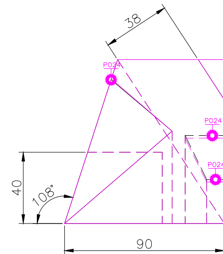
RIGHT SCALE 1/2
