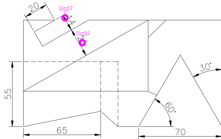
TOP SCALE 1/2
