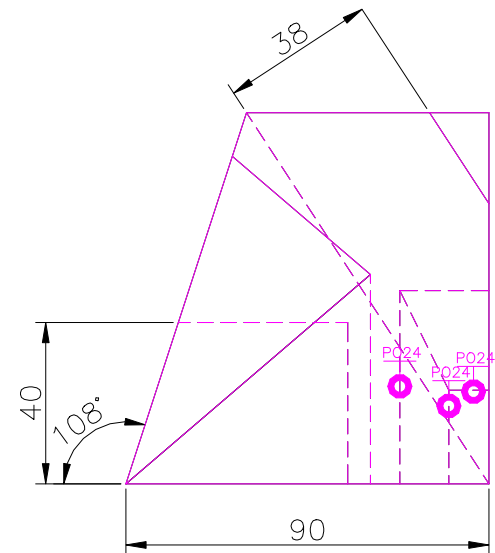
RIGHT SCALE 1/2
