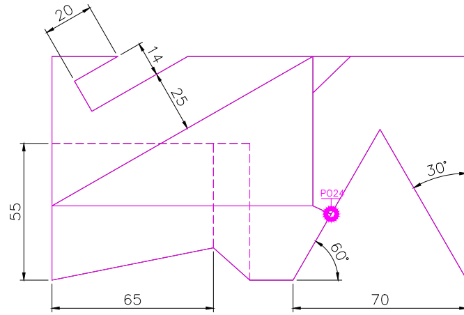
TOP SCALE 1/2
