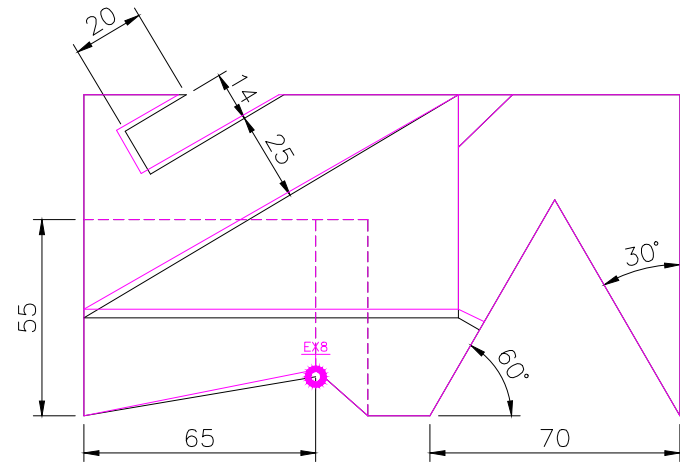
TOP SCALE 1/2
