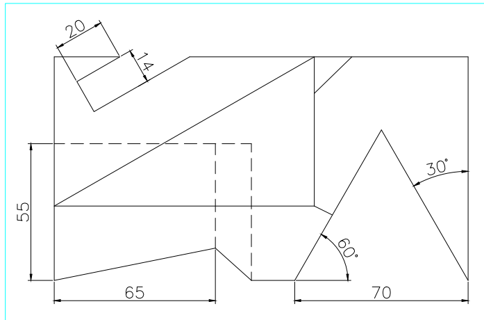
TOP SCALE 1/2
