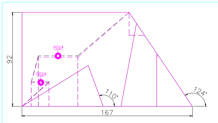
FRONT SCALE 1/2
