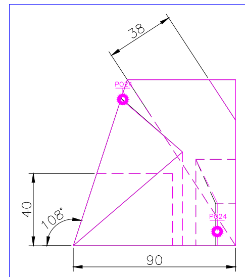
RIGHT SCALE 1/2
