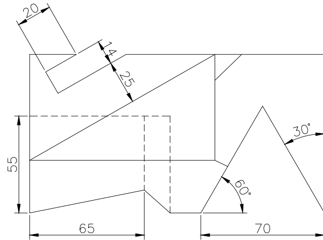
TOP SCALE 1/2
