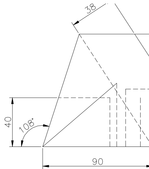
RIGHT SCALE 1/2
